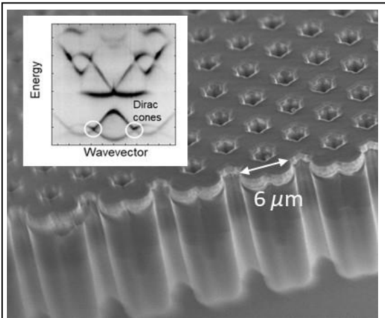
Electron microscopy image of a honeycomb lattice of semiconductor resonators, which emulate graphene physics. Inset: band structure measured by optical spectroscopy revealing characteristic Dirac cones.
